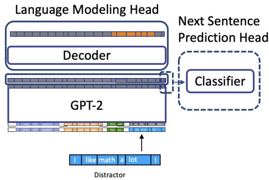
Figure 2: Two model heads—one for language modeling to generate responses with high quality in grammatical and semantical aspects, and one for next-sentence prediction to ensure the match between the generated responses and the context input. Adapted from Wolf [42].
