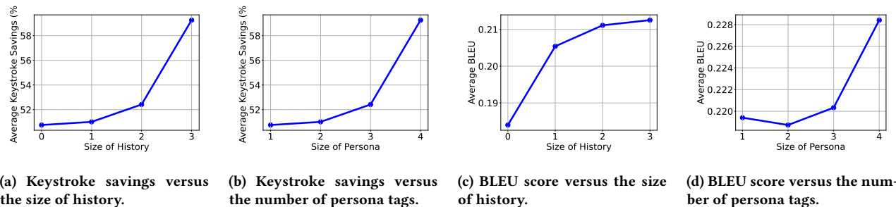
Figure 7: Benefits of increasing the size of history (number of exchanges in conversation history) and persona tags. More history and persona tags help the language generation model to output higher quality responses.
