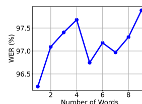
Figure 9: Average WER score against the number of words for the left-to-right sentence generation model. This result suggest that this model is not usable as the generated sentences are not valid.
