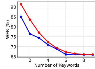
Figure 5: The blue line plots the average WER of generated sentence with respect to the target sentence against the number of keywords input to the model. The red line represents the WER from just entering the keywords without feeding them to the KWickChat language generation model to form a complete sentence. Just entering keywords approaches the generated sentences when the number of keywords is large, because WER only measures word-level similarity.
