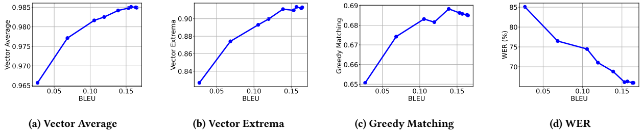
Figure 6: Correlation between BLEU and different metrics. The three embedding-based metrics all share a positive correlation with BLEU and a negative correlation with WER.
