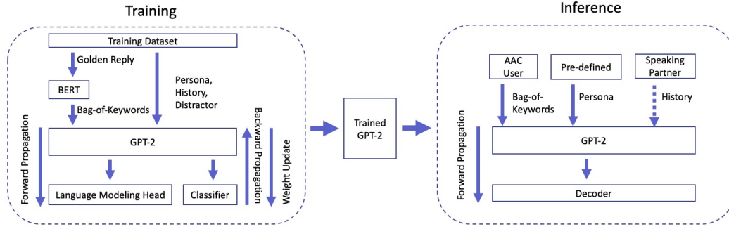
Figure 3: The overall process flow of the proposed KWickChat language generation model. Firstly, a GPT-2 is trained/fine-tuned using the ConvAI2 challenge dataset as the training dataset. The trained/fine-tuned GPT-2 model is then used to perform inference from the inputs including bag-of-keywords, persona and history to generate high-quality responses. Note that the history does not only come from the speaking partner but also from the system itself, which are the selected responses by the AAC user.
