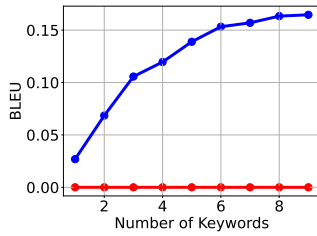
Figure 4: The blue line plots the average BLEU of the generated sentence with respect to the target sentence against the number of keywords input to the model. The red line plots the BLEU score from just entering the keywords without feeding them to the KWickChat language generation model to form a complete sentence. The more keywords the user enters, the better the quality of the generated response. The reference score from the keywords stays close to zero as keywords do not form a sentence, and BLEU uses n-gram modeling to measure the similarity with the generated response.
