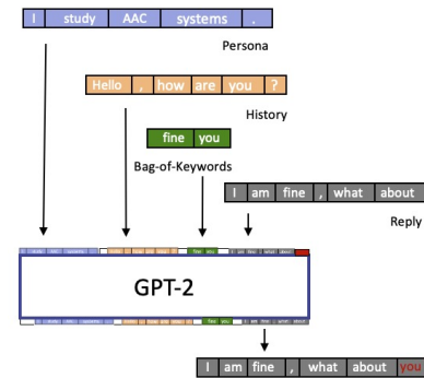
Figure 1: The four context segments are concatenated and used as the input to the GPT-2. Another input is the segment embeddings which are represented by the different colors. The predicted tokens, indicated by the red segment and red text in the figure, are used as the last segments in the concatenated segments to enable token-by-token prediction. Adapted from Wolf [42].
