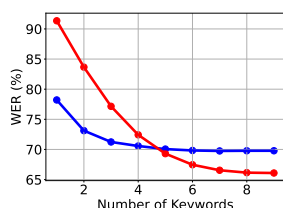
Figure 8: The blue line represents the average WER score against the number of keywords for TF-IDF. The red line represents the WER score based on raw keywords. The improvement from the increase in the number of keywords is marginal and soon saturates at four keywords.
